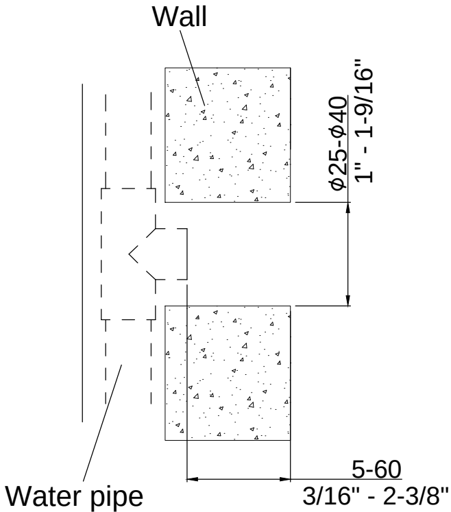
Layout for water pipe
