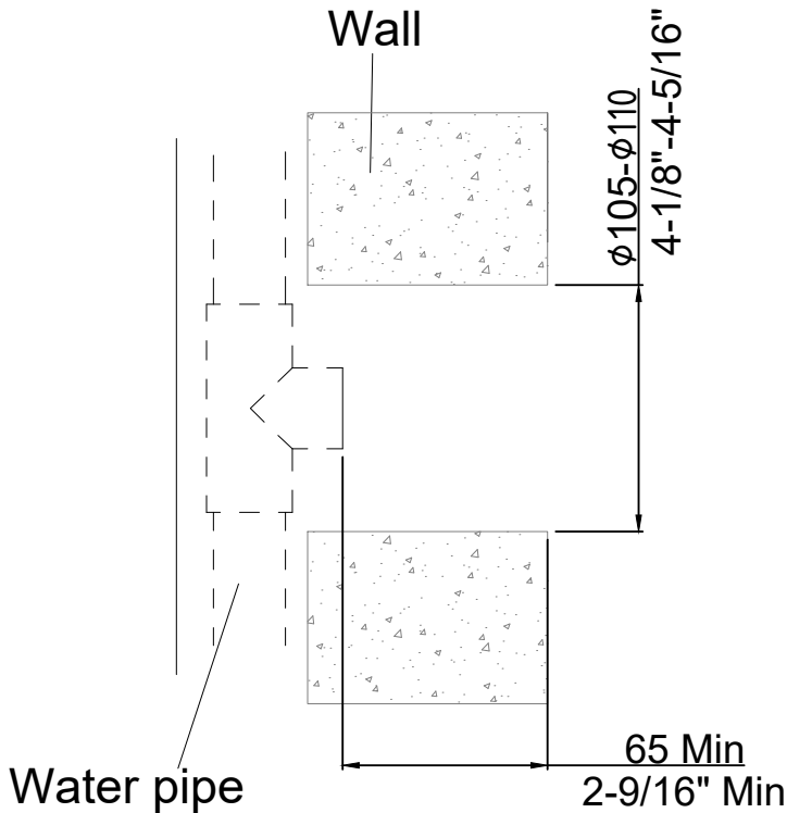
Layout for water pipe
