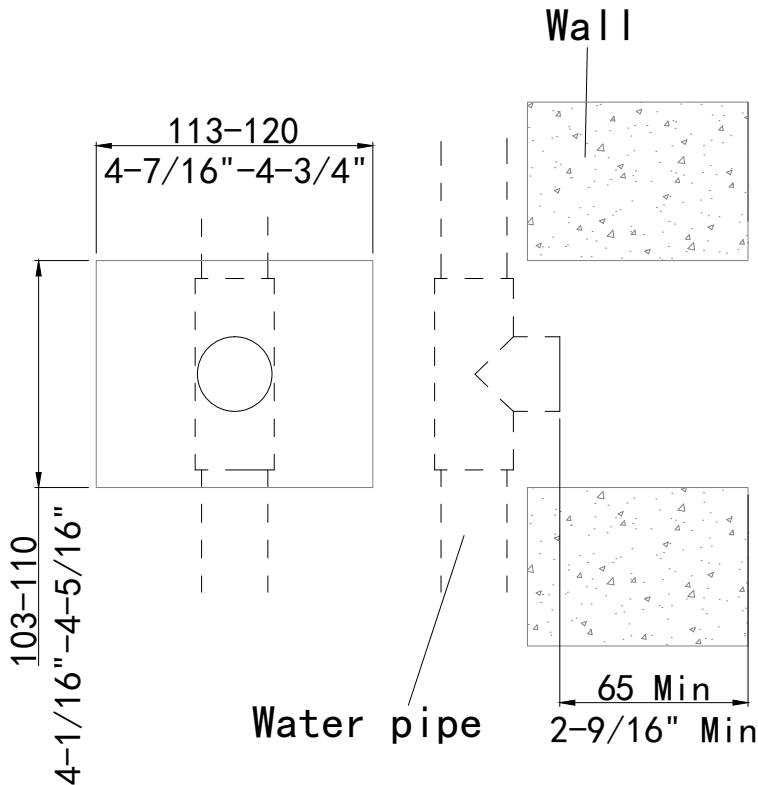
Layout for water pipe
